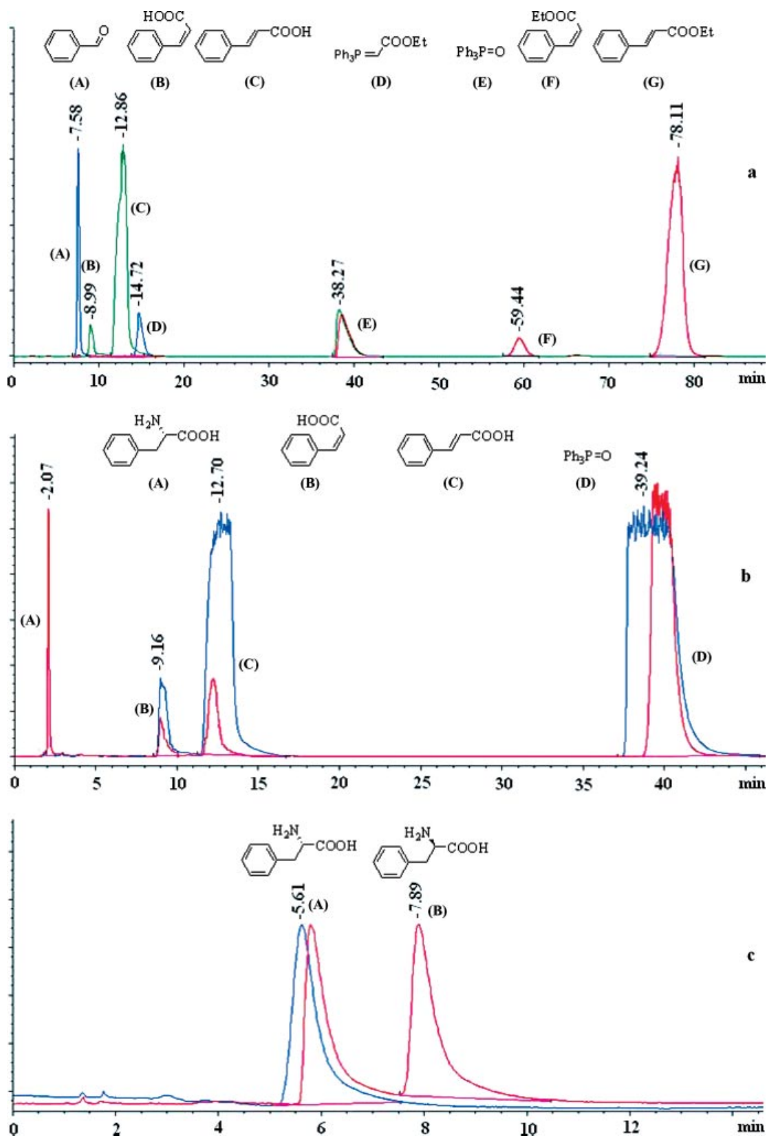
Figure 1. (a) Elution diagram of the starting materials (blue trace) and the products of the Wittig (red trace) and PLE-mediated reactions (green trace). (b) Elution diagram of the products of the two enzymatic steps of the one-pot reaction: PLE-mediated (blue trace) and PAL-catalysed (red trace). (c) Elution diagram of the isolated product of the one-pot reaction, L-phenylalanine (blue trace) and ( rac )-phenylalanine as reference (red trace).
