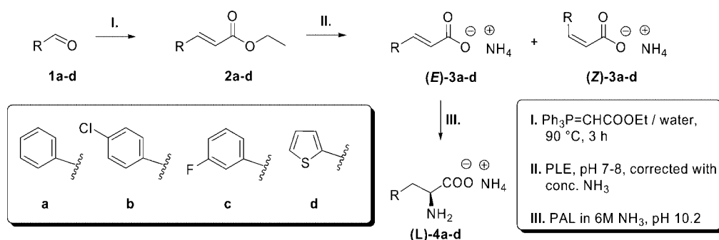
Scheme 1. The one-pot synthesis of L-arylalanines.
